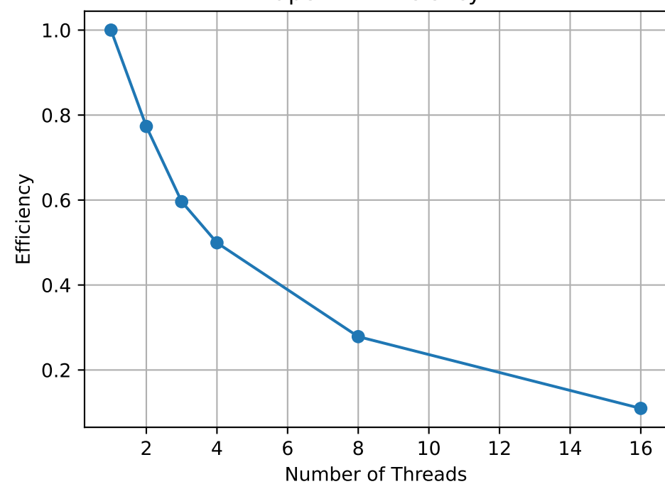
OpenMP Efficiency
