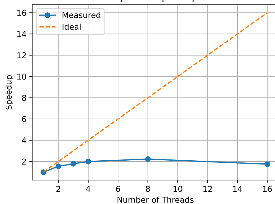
OpenMP Speedup
